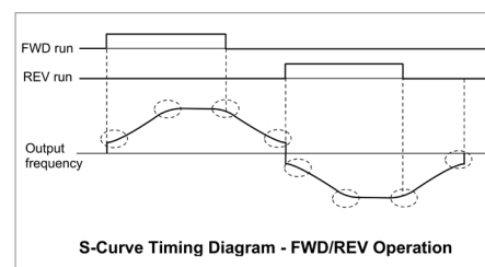
Figure 4: Accel/Decel curves
