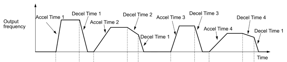
Figure 3: Output frequency vs. time showing acceleration and deceleration times
