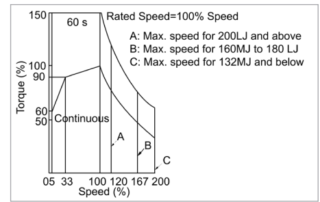
Figure 2: Typical Speed Torque Curve, showing overload conditions
